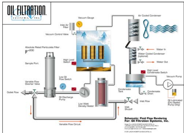
Vacuum Dehydrator Process Diagram
